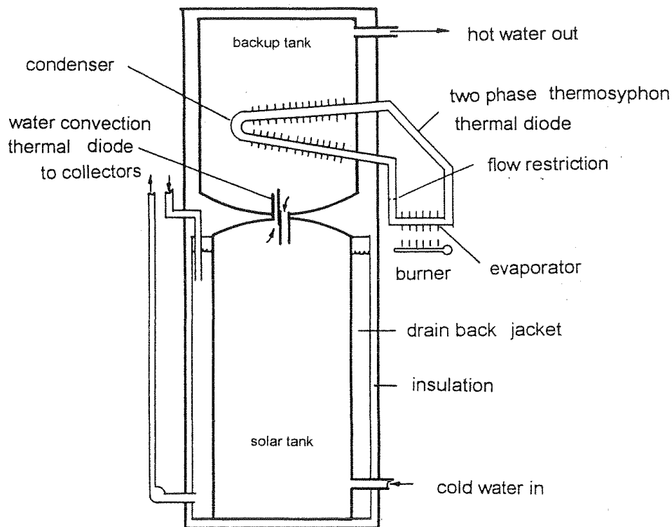
Figure 1. Cross Section of Our Current (Grunes et al, 1982) Solar-Augmented Gas-Fired Water Heater
